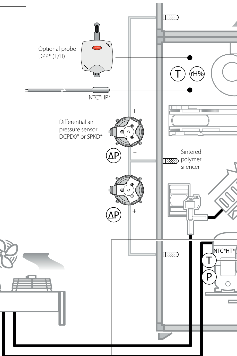
BLDC compressor
